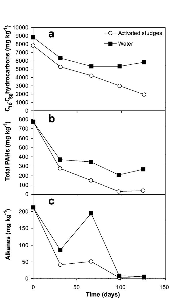
Figure 2. Monitoring of hydrocarbons in biopiles. Each biopile received activated sludge or water. (a) \text{C}_{10}\text{-C}_{50} hydrocarbons. (b) Total PAHs. (c) Alkanes.
