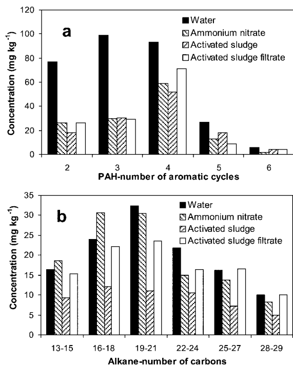
Figure 1. Concentration of hydrocarbons in microcosms after 15 days of incubation. Microcosms received sludge, sterile sludge filtrate, ammonium nitrate or water. (a) Concentration of PAHs. (b) Concentration of alkanes.
