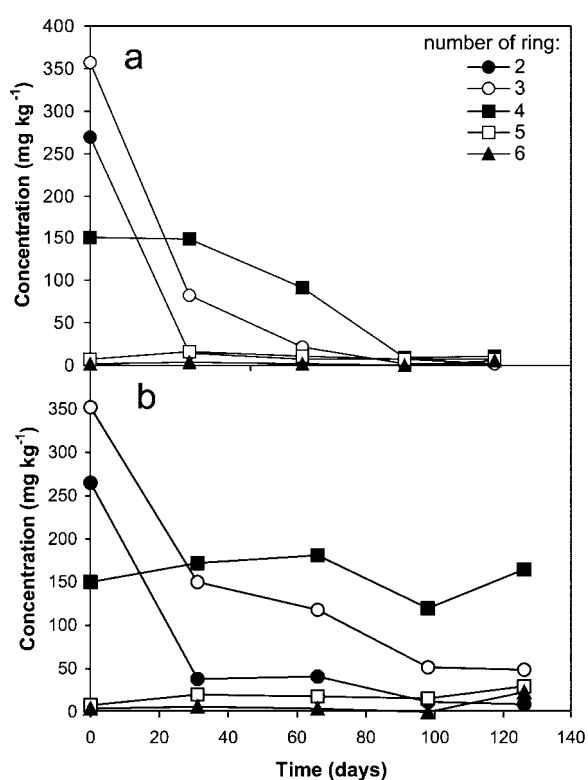
Figure 3. Monitoring of PAHs in biopile as function of their number of cycle. (a) Biopile that received activated sludge. (b) Biopile that received water only.
